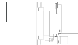
Blockzarge 60 mm
